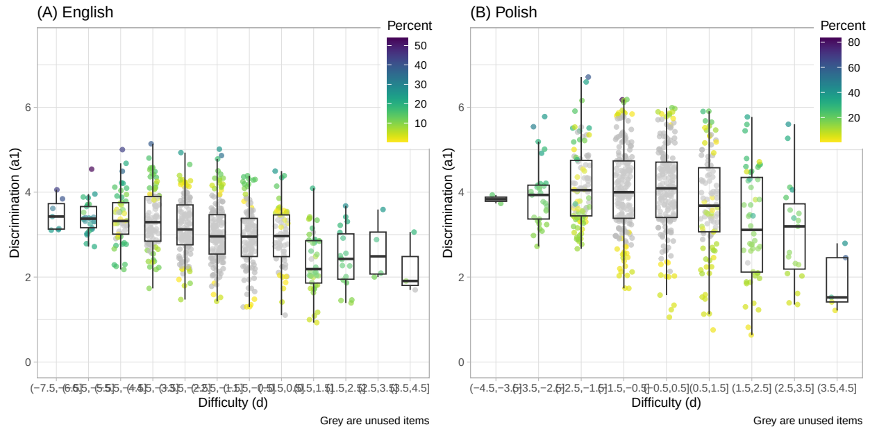
Figure 5. How often a given item was used in CAT-CDI administrations in the validation study in (A) English and (B) Polish. The items (points) are colored by the percentage of their appearance in the CAT-CDI administrations. Items colored in grey are items never used in any of the CAT-CDI administrations.
