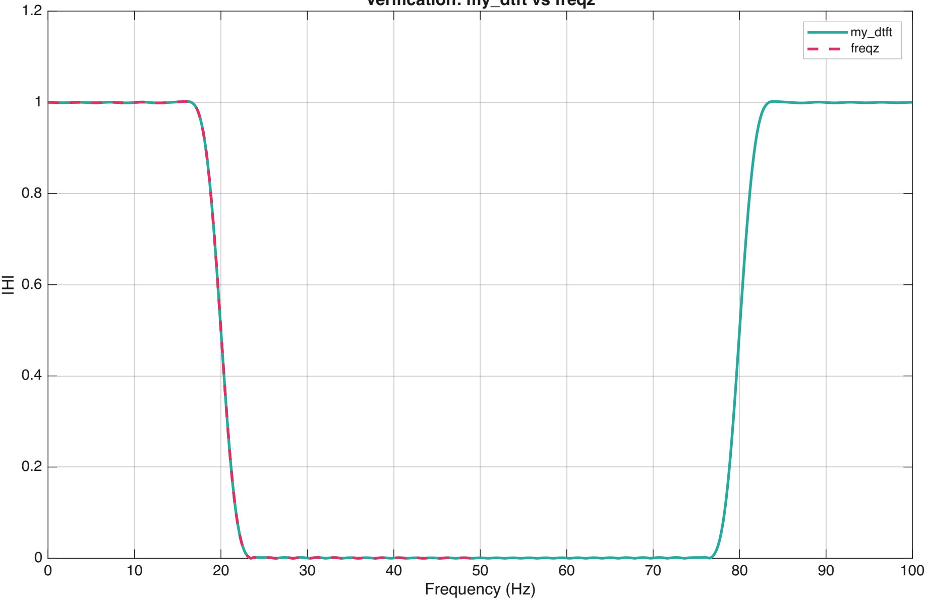
Verification: my_dtft vs freqz
