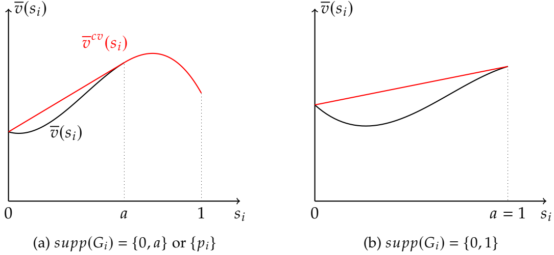
Figure 1: Illustration of Lemma 1 (ii)
