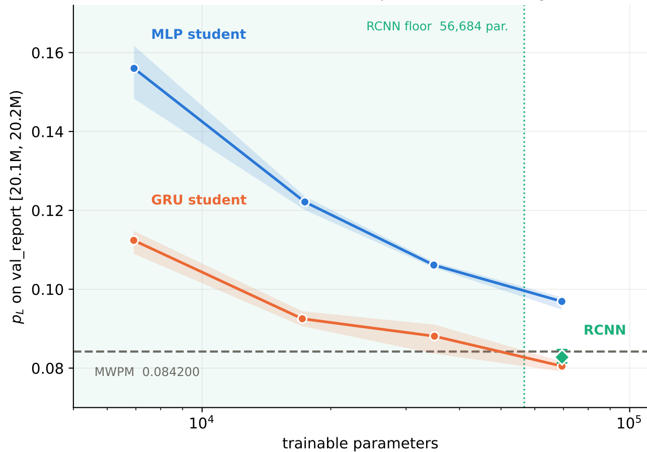
Parameter-reduction curves — d=5 , r=5 , p=0.010 , 10M training shots
