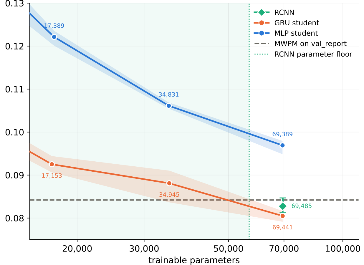
Parity region
