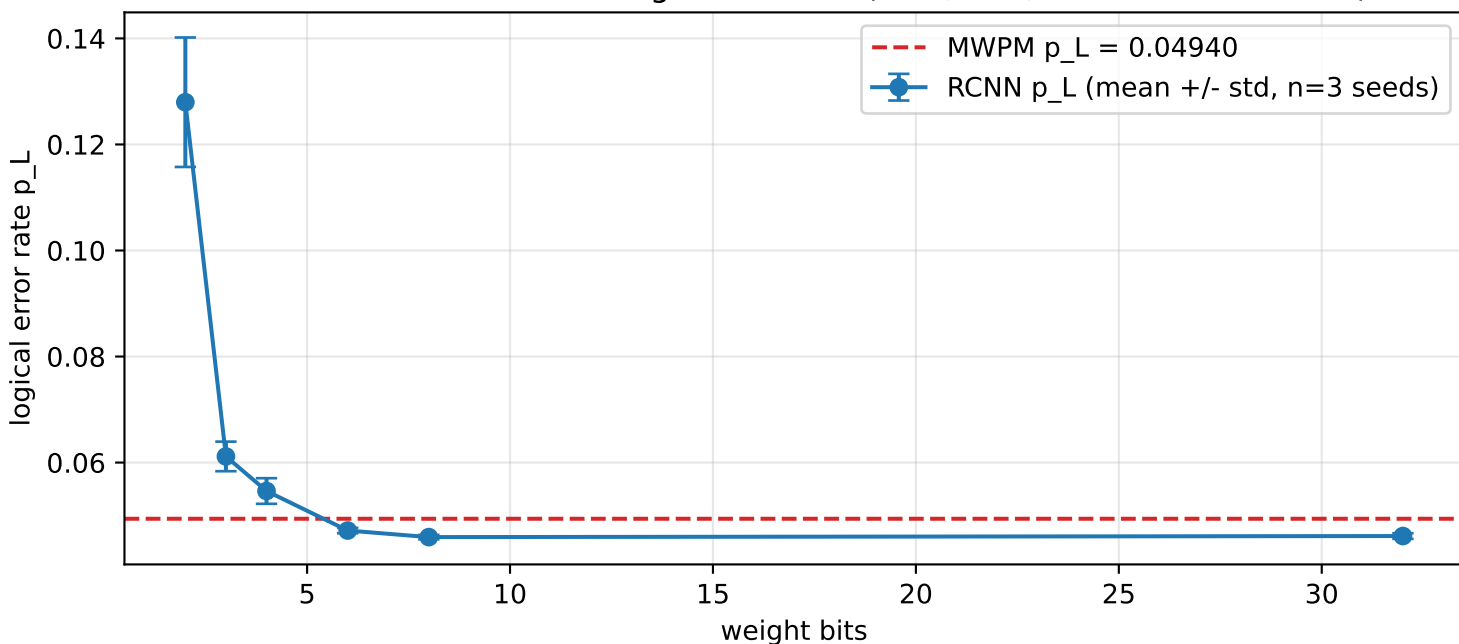
RCNN vs MWPM across weight bit-width (d=5, r=3, fresh 200k-shot tail)
