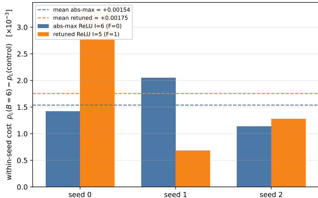
Phase 2a-ReLU: B=6 activation cost vs decoder-ReLU integer width lowering I=6->5 (frac 0->1) did NOT reduce the cost -- seeds move both ways, mean unchanged
