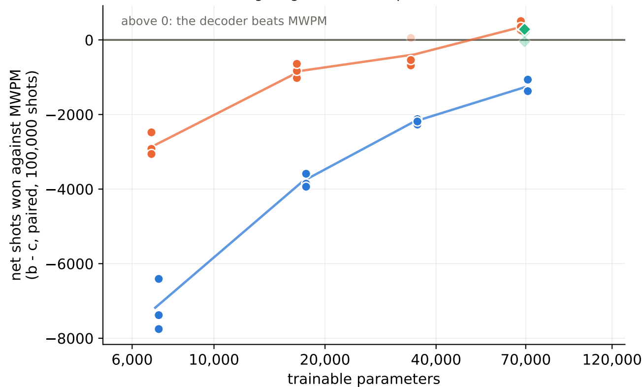
Paired McNemar margin against MWPM, per seed
