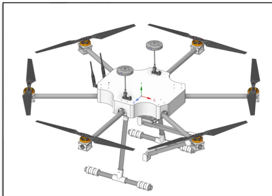
Designed developed Anomaly detection drone with protracting arm
