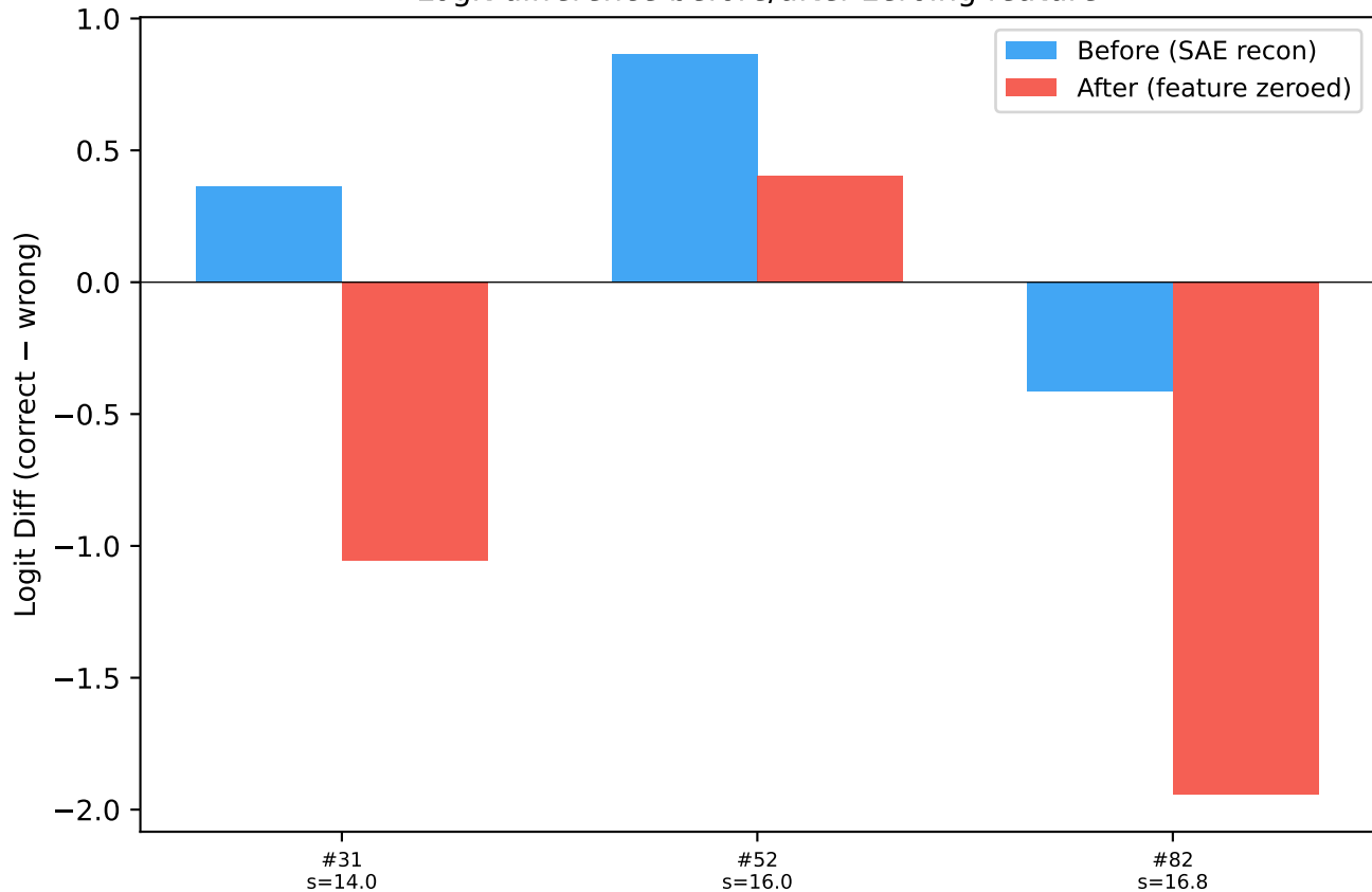
L10 Feature 2046 (aligned: " de") Logit difference before/after zeroing feature
