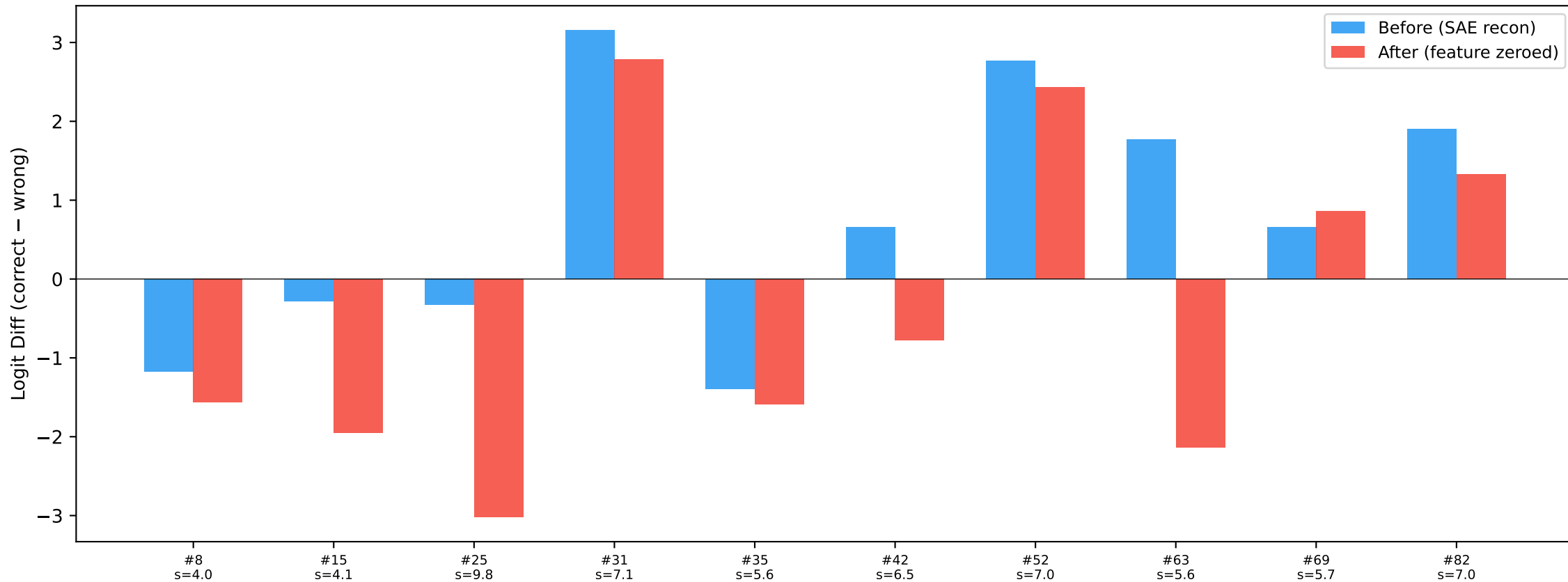
L1 Feature 3590 (aligned: "ts") Logit difference before/after zeroing feature
