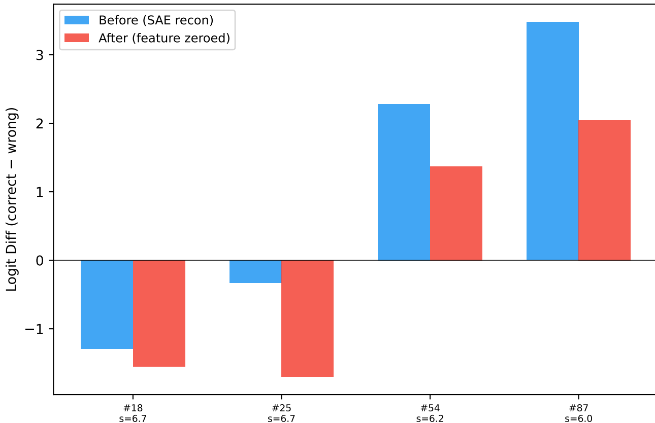
L1 Feature 3617 (aligned: "berg") Logit difference before/after zeroing feature
