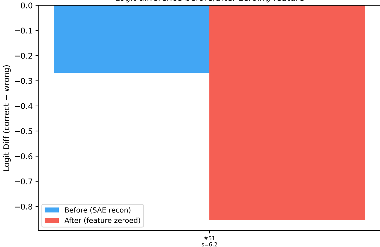
L3 Feature 2842 (aligned: "studio") Logit difference before/after zeroing feature
