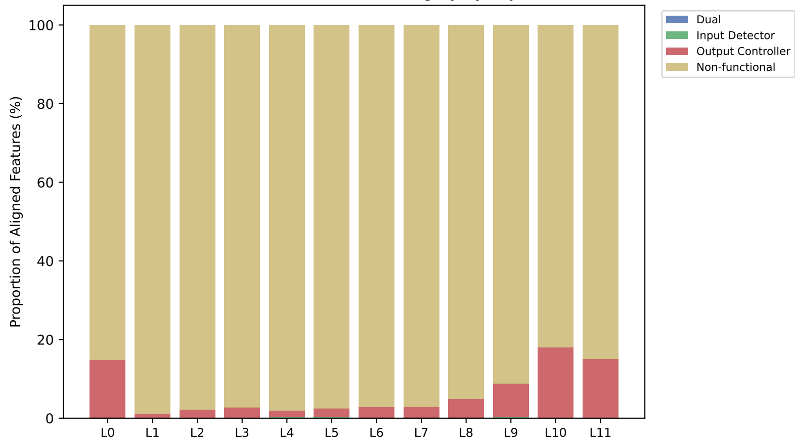
GPT-2: Feature Functional Category by Layer
