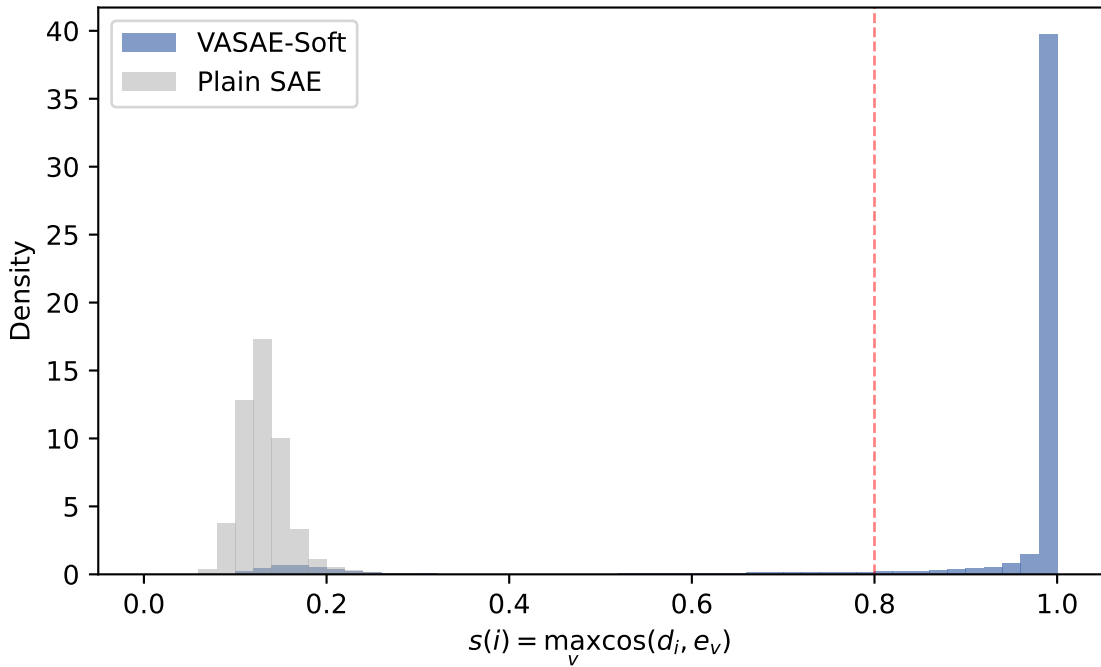
GPT-2: Overall Geometric Alignment Distribution
