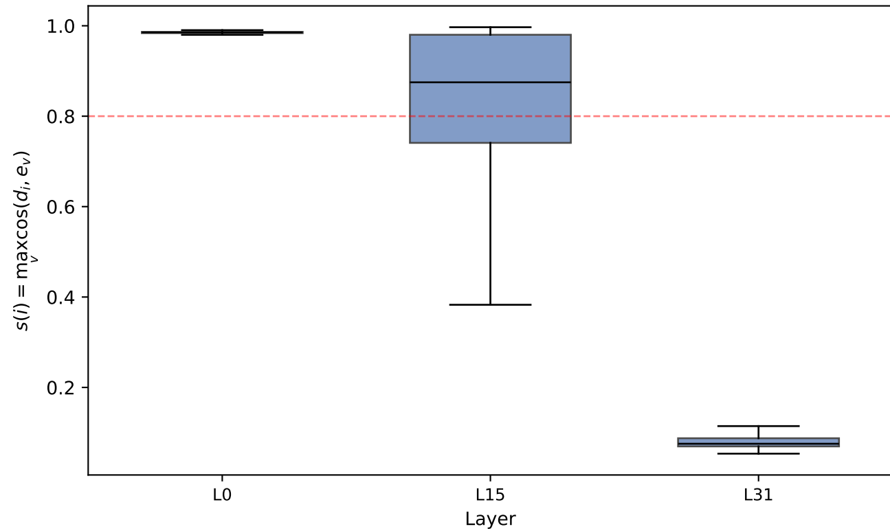
Llama-3.1-8B ( \lambda=5e-3 ): Geometric Alignment by Layer
