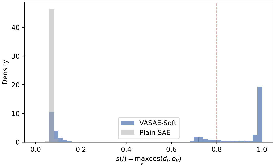
Llama-3.1-8B ( \lambda=5e-3 ): Overall Geometric Alignment Distribution
