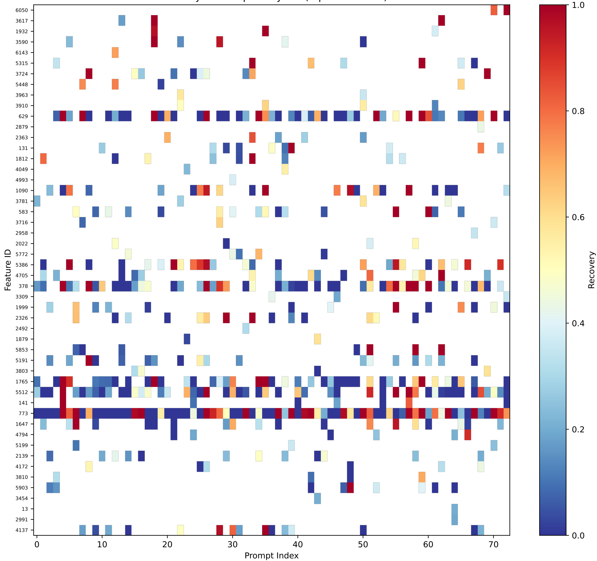
Recovery Heatmap — Layer 1 (top 50 features)
