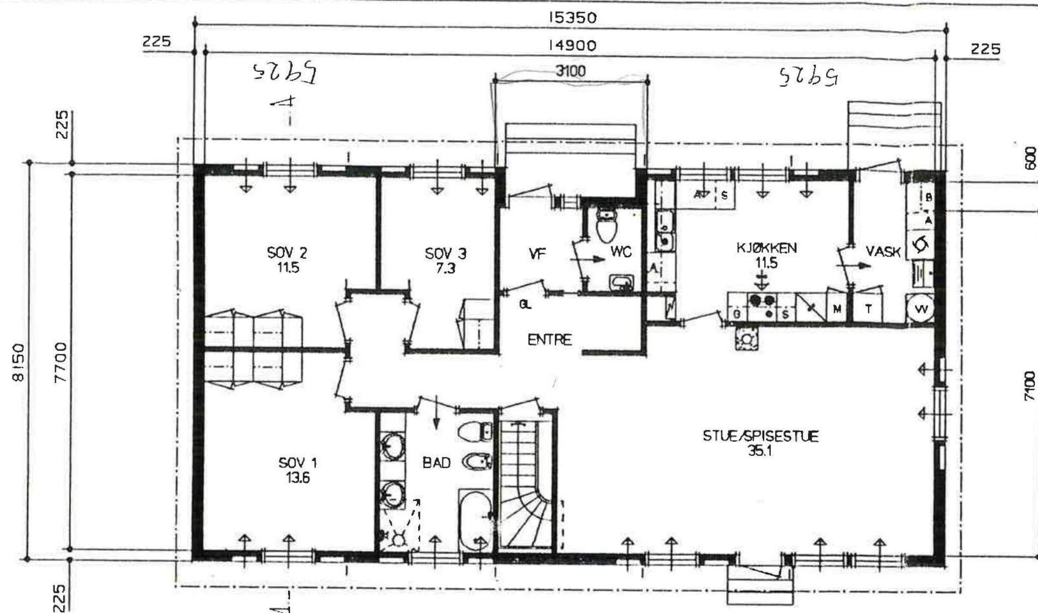
PLAN MK.410.07-P-MOD
