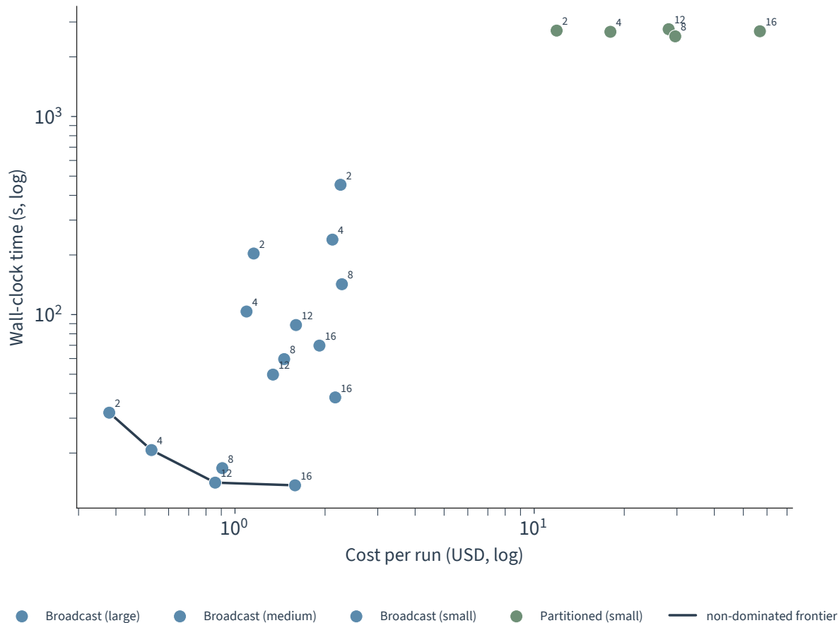
Cost-time tradeoff of the distributed join
