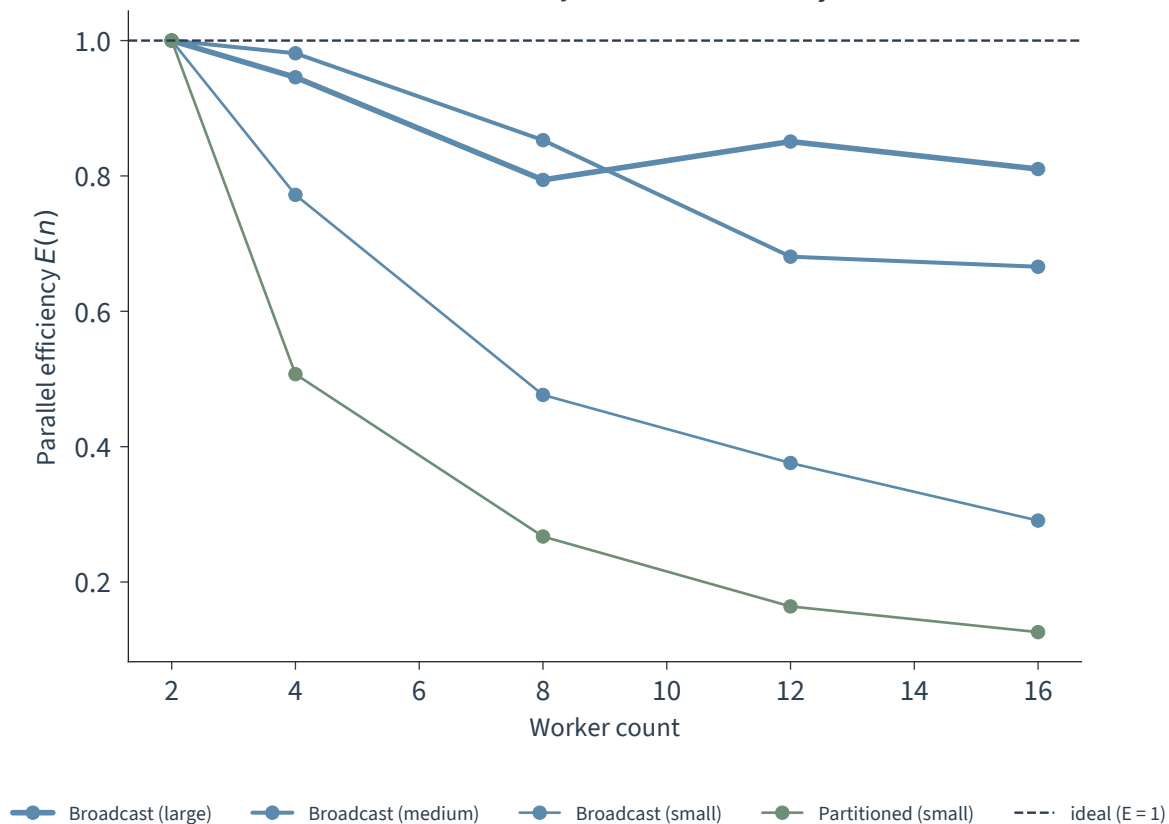
Parallel efficiency of the distributed join
