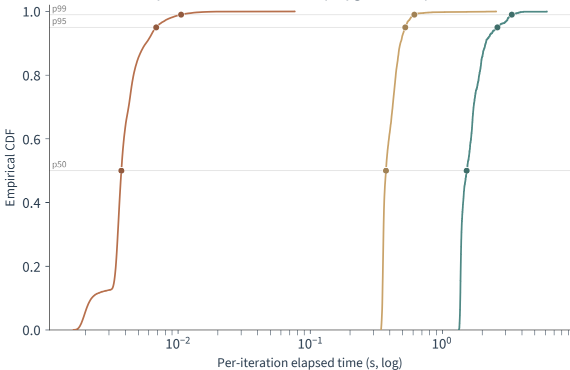
Latency distribution — Point-in-polygon Lookup (small tier)
