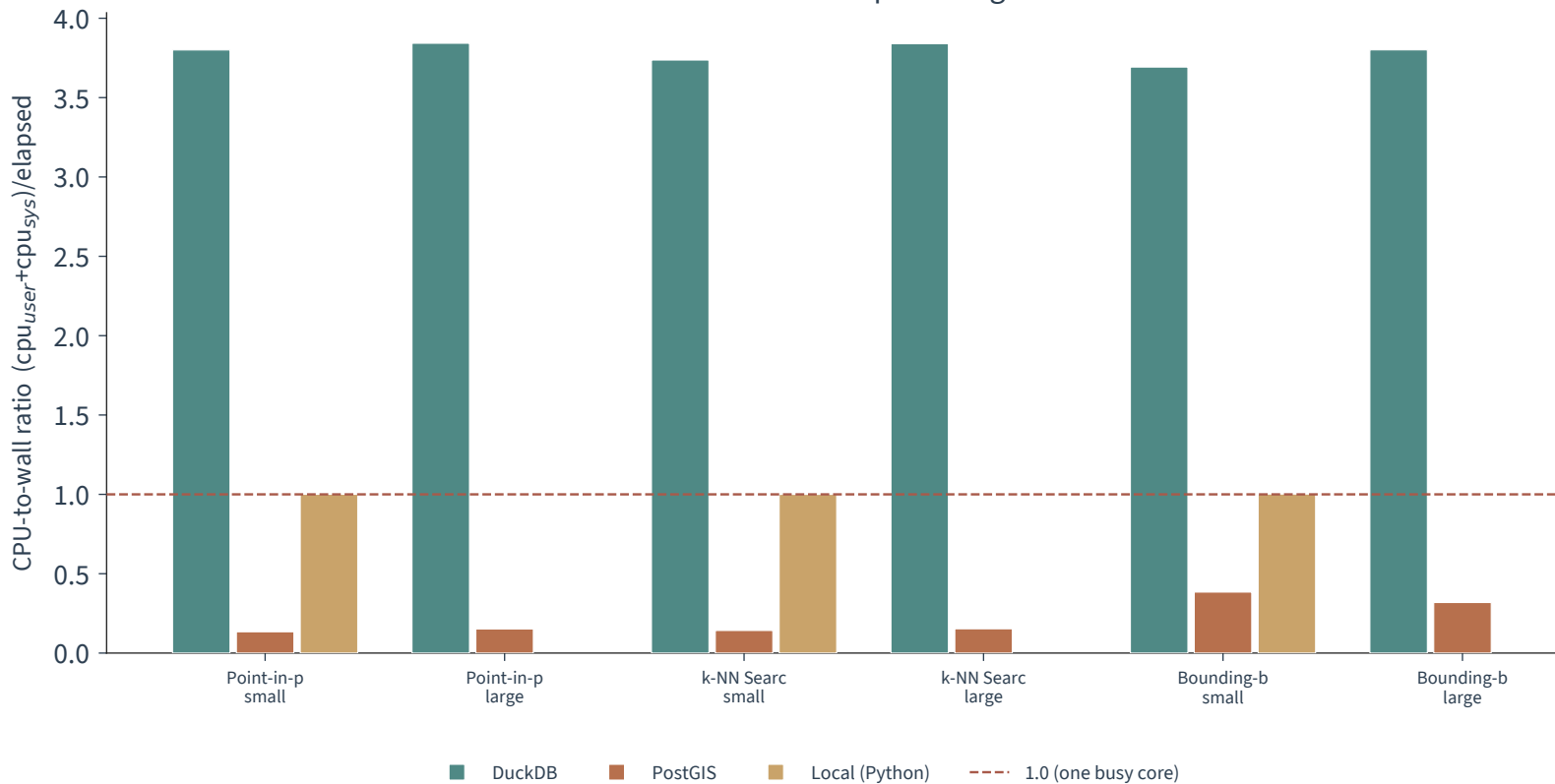
CPU-to-wall-clock ratio per configuration
