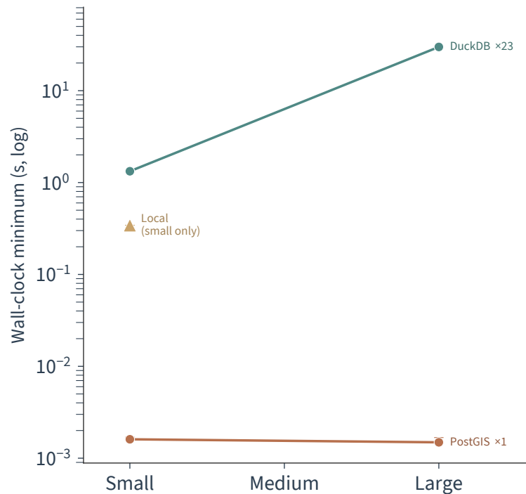
Point-in-polygon Lookup
