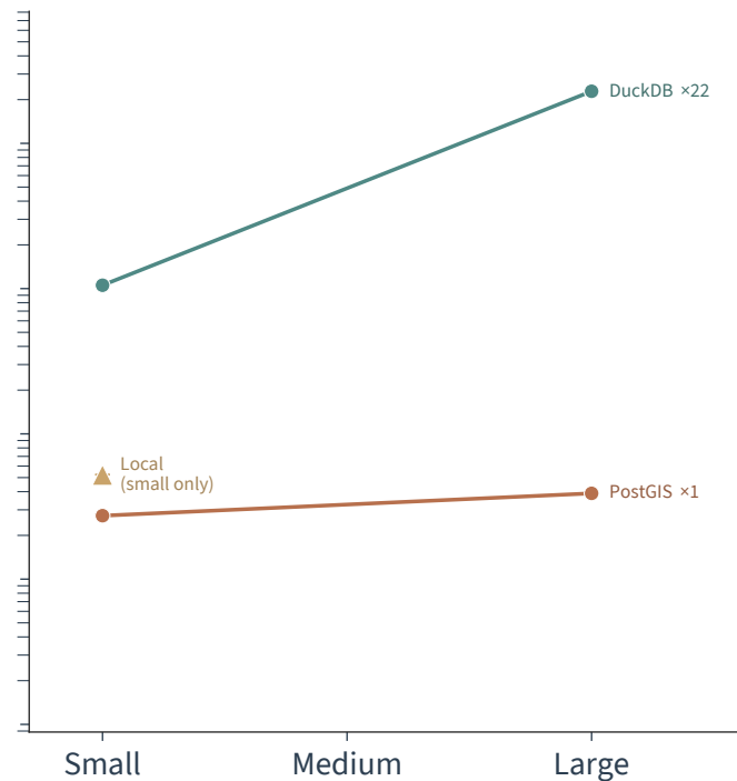
Bounding-box Filtering
