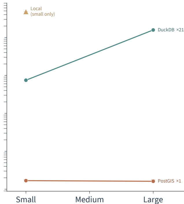
k-NN Search
