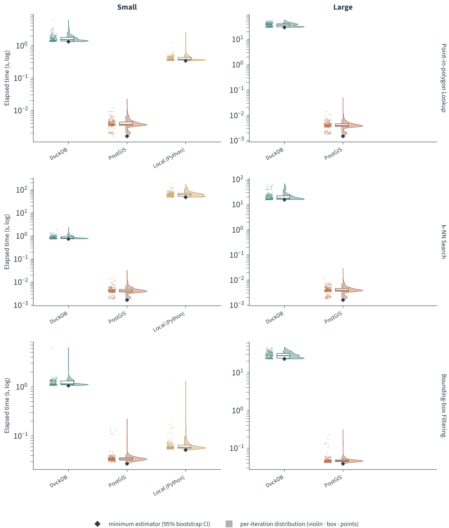
Wall-clock time per single-machine configuration (minimum estimator)
