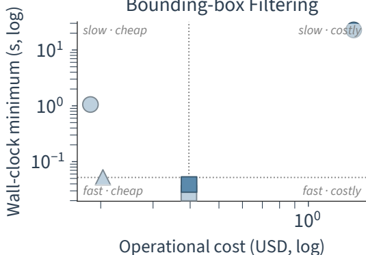
Bounding-box Filtering
