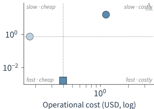
k-NN Search
