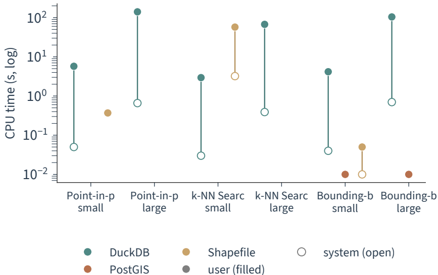
CPU-time decomposition (user vs system, median)
