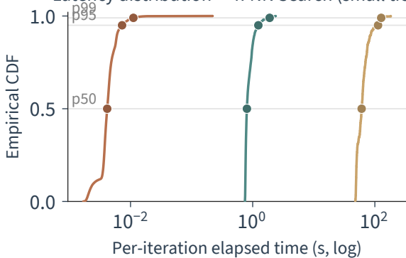
Latency distribution — k-NN Search (small tier)
