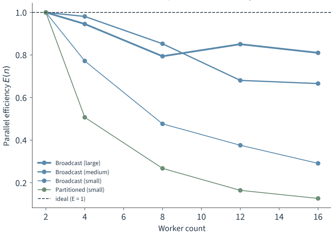
Parallel efficiency of the distributed join
