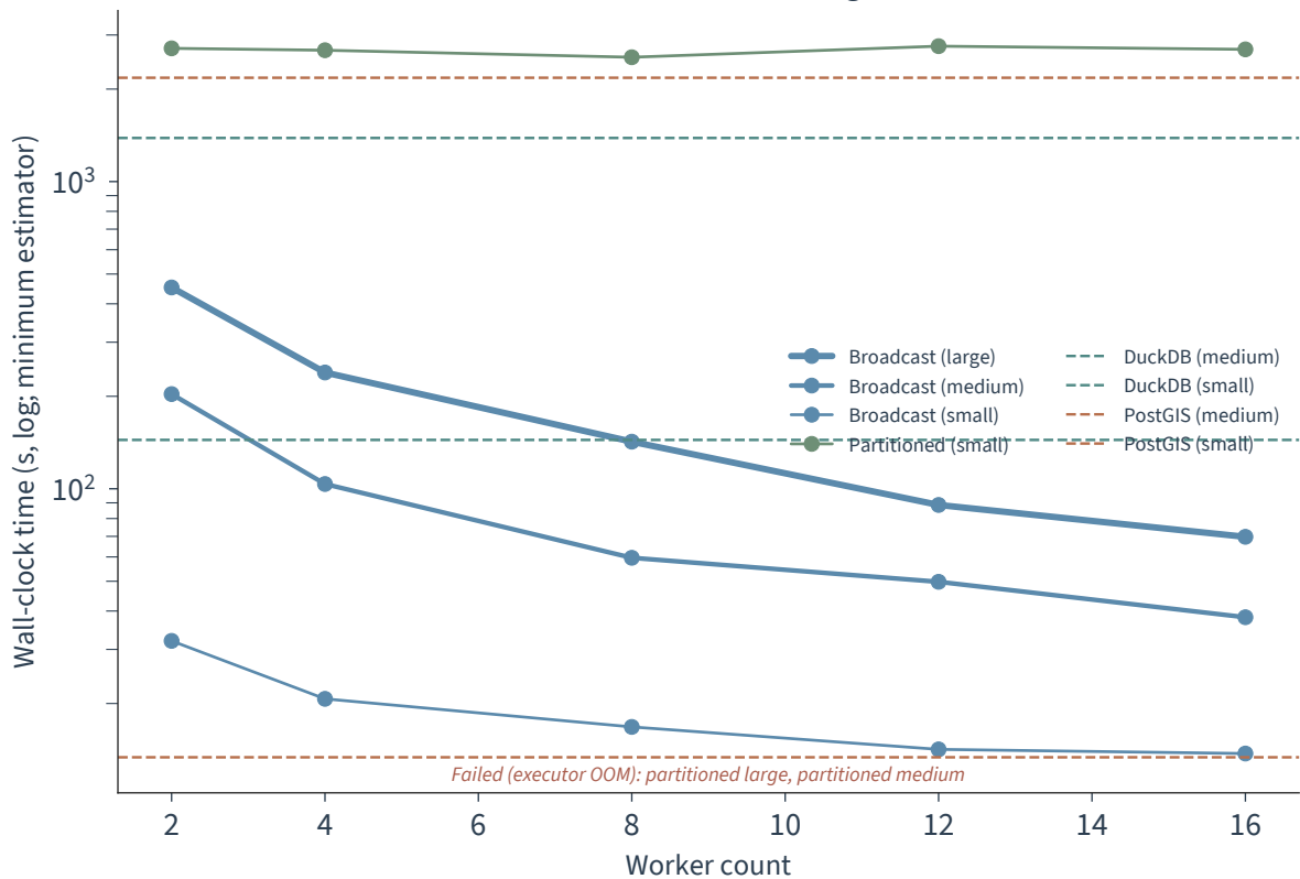
Distributed wall-clock time versus single-node baselines
