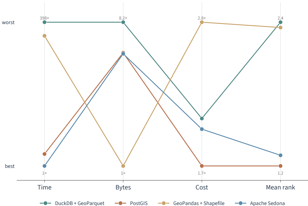
Per-system outcomes across dimensions (parallel coordinates)
