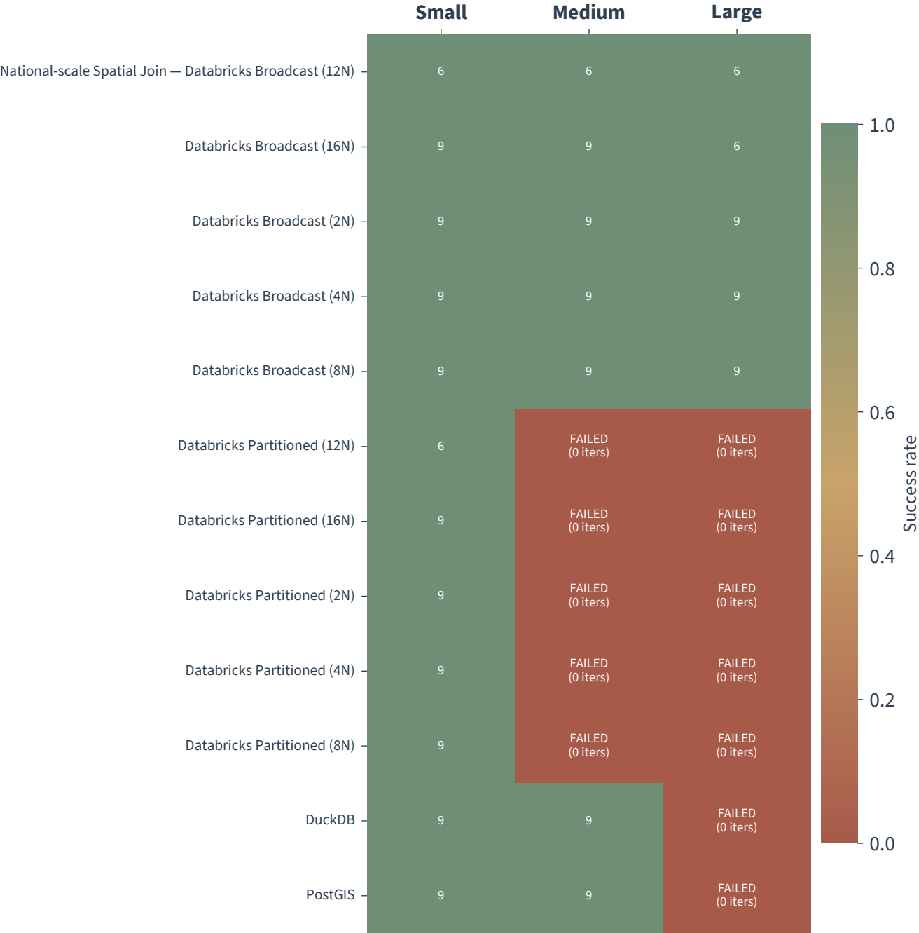
Distributed-join benchmark coverage — success rate by configuration
