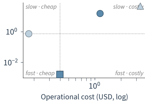
k-NN Search
