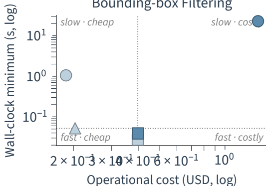
Bounding-box Filtering
