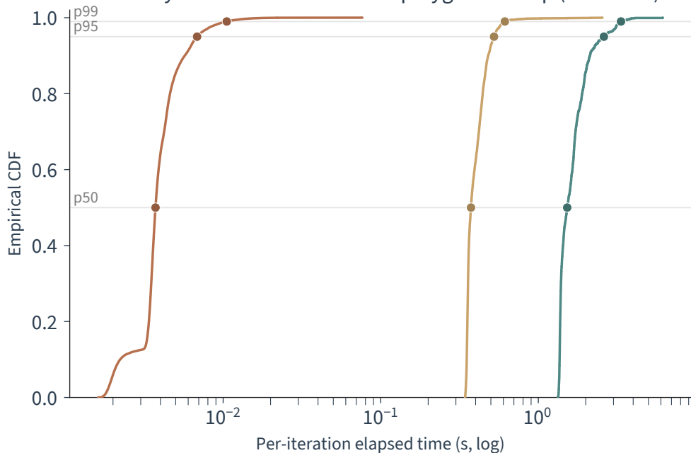
Latency distribution — Point-in-polygon Lookup (small tier)
