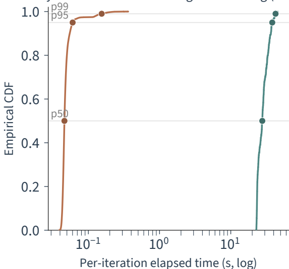
Latency distribution — Bounding-box Filtering (large tier)
