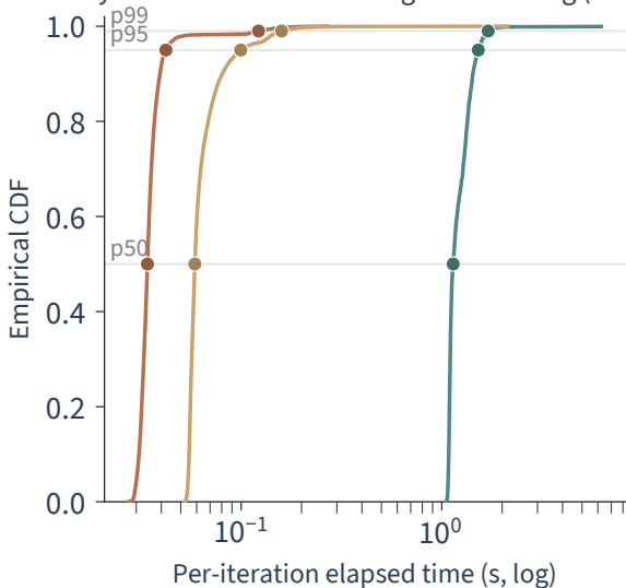
Latency distribution — Bounding-box Filtering (small tier)
