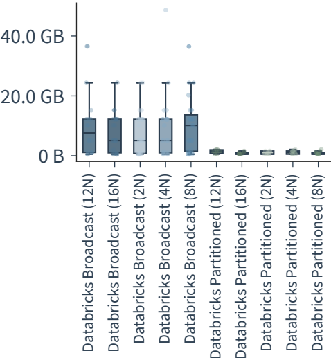
Executor input bytes read
