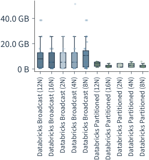
Shuffle write (bytes)
