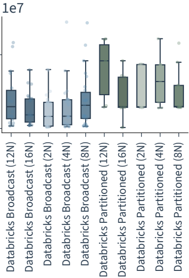
Executor run time (ms)
