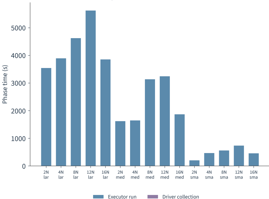
Execution-phase wall-clock time (broadcast)
