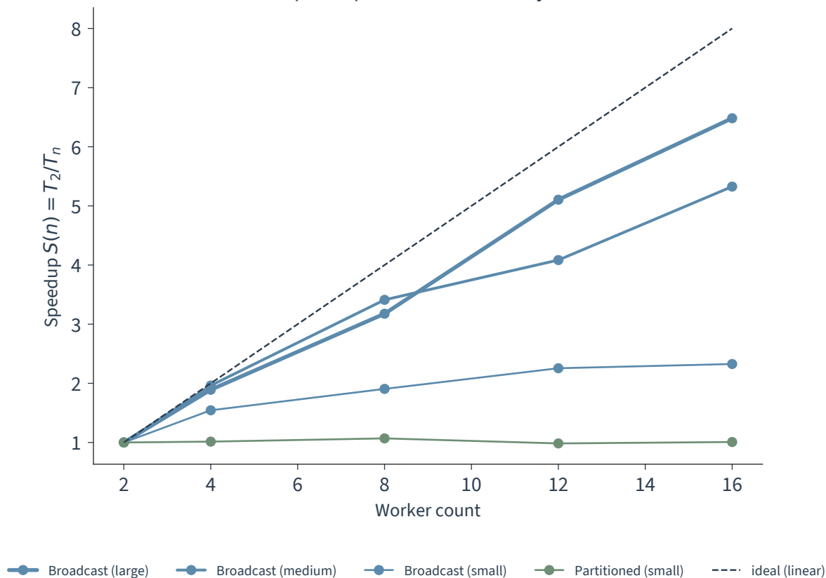
Speedup of the distributed join
