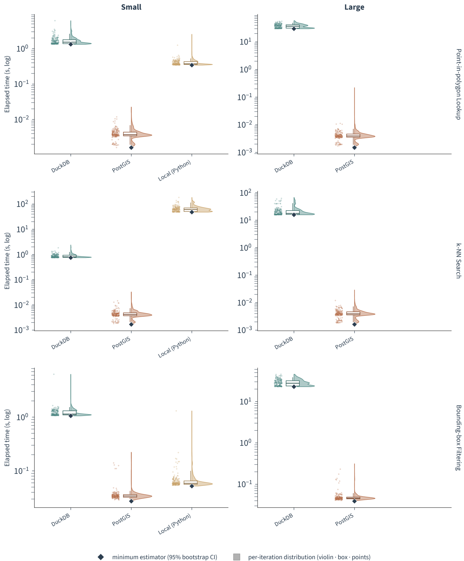
Wall-clock time per single-machine configuration (minimum estimator)
