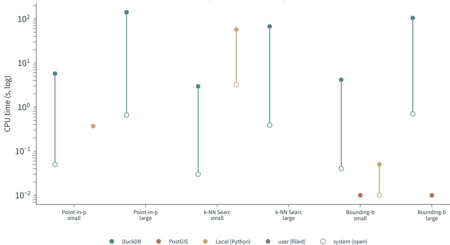
CPU-time decomposition (user vs system, median)
