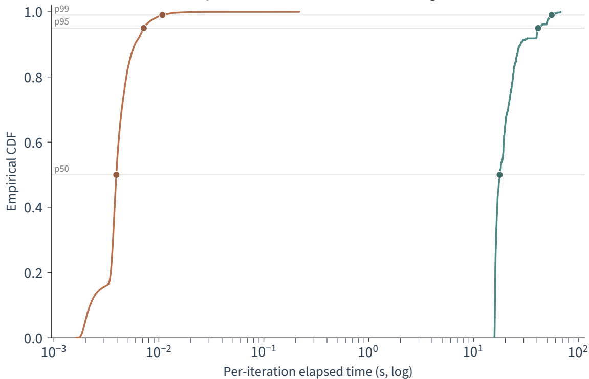
Latency distribution — k-NN Search (large tier)
