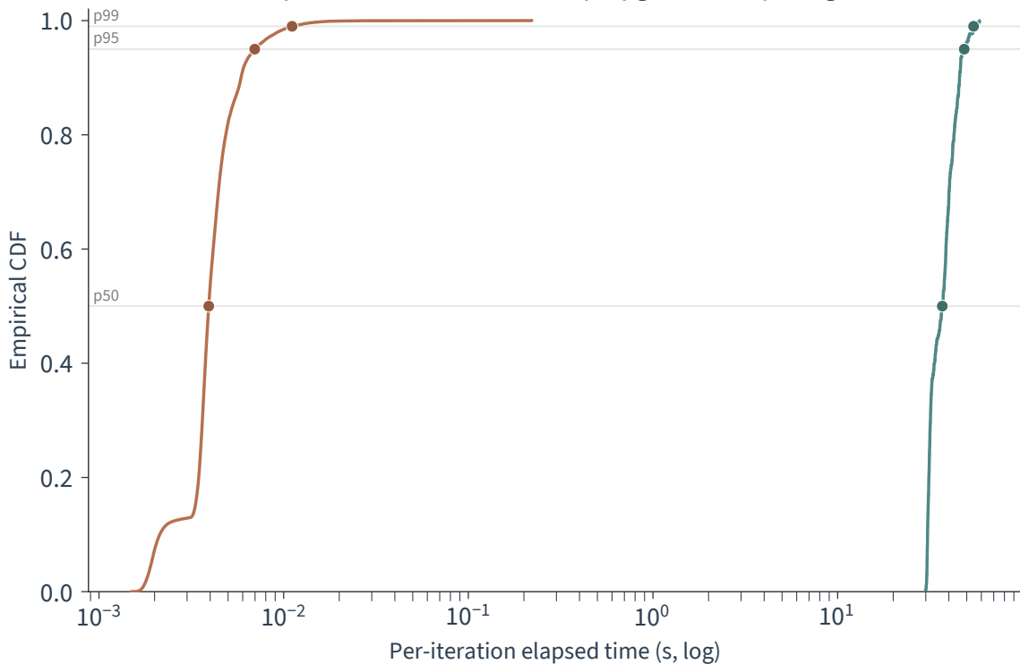
Latency distribution — Point-in-polygon Lookup (large tier)
