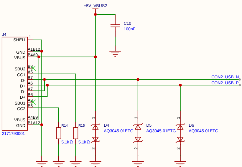
USB-C CONNECTOR 2
