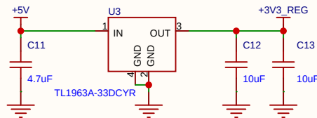
5V TO 3V3
