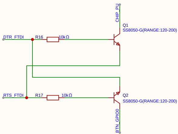
SERIAL SIGNALS HANDLING
