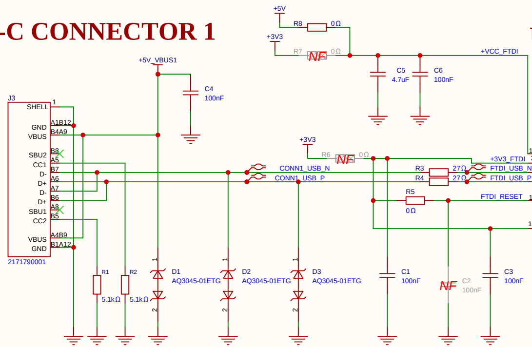
USB TO UART
