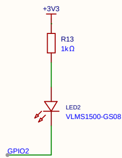
USER LED
