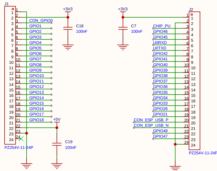
HEADERS
