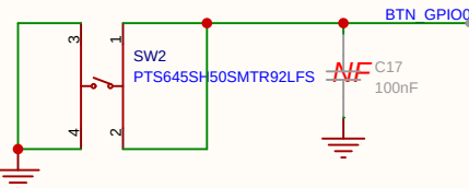
BOOT / USER BUTTON
