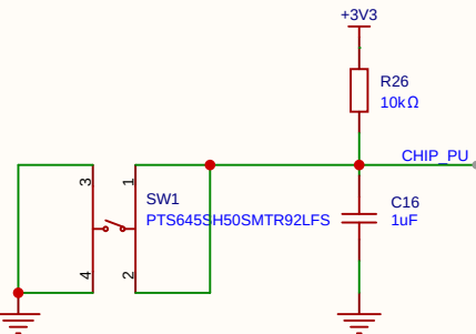
RESET BUTTON
