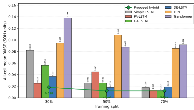
Figure 3: Mean RMSE of six single-cell predictors and the proposed hybrid across the 30%, 50% and 70% splits.
