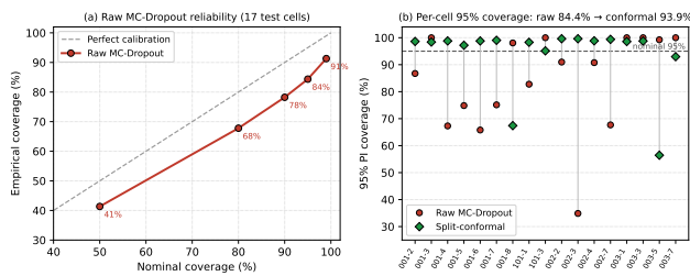
Figure 11: Uncertainty calibration on the 17 test cells.
