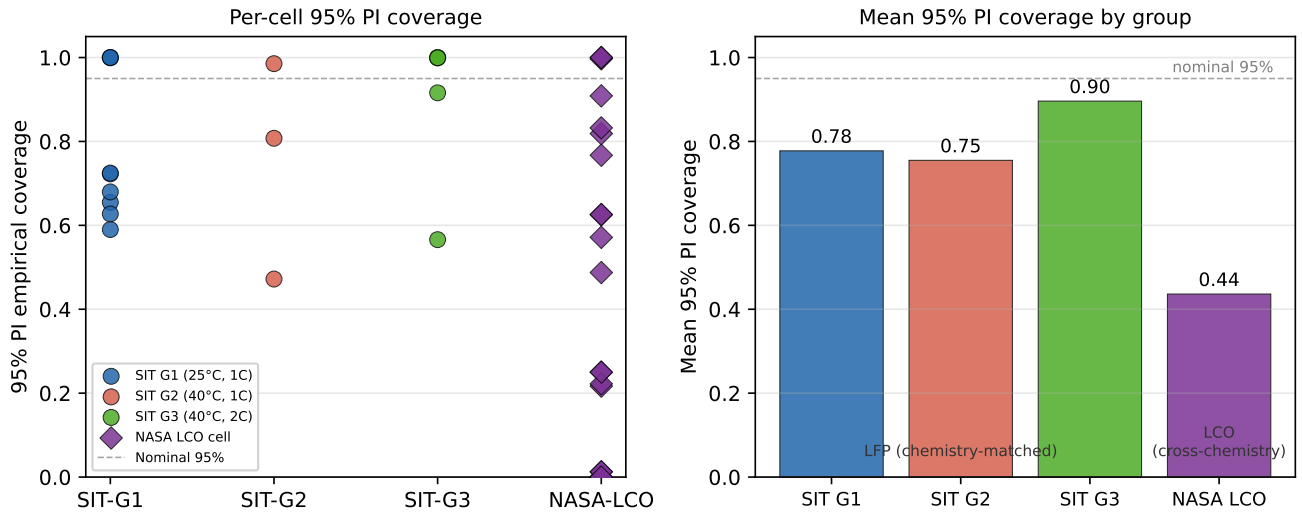
Figure 12: MC-Dropout 95% PI empirical coverage by dataset and group.
