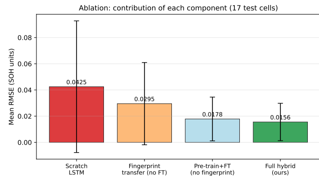
Figure 8: Ablation study: mean RMSE per configuration (50% split).
