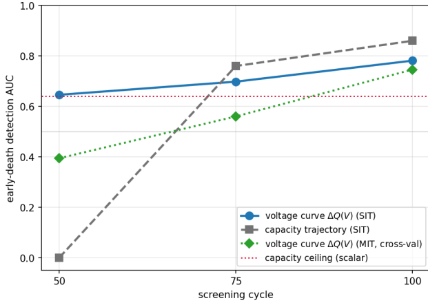
Figure 14: Early detection AUC versus screening cycle.
