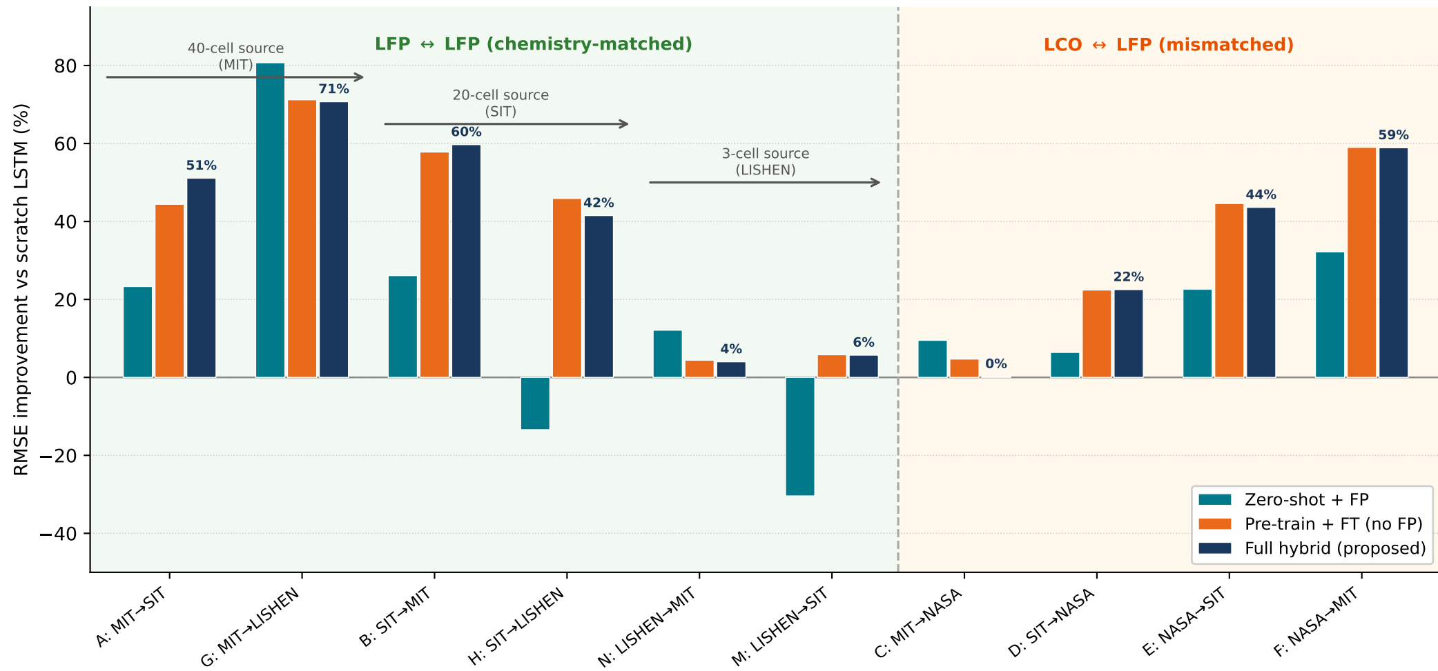
Cross-Dataset Transfer: RMSE Improvement by Scenario and Configuration
