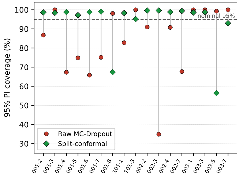
(b) Per-cell 95% coverage: raw 84.4% → conformal 93.9%
