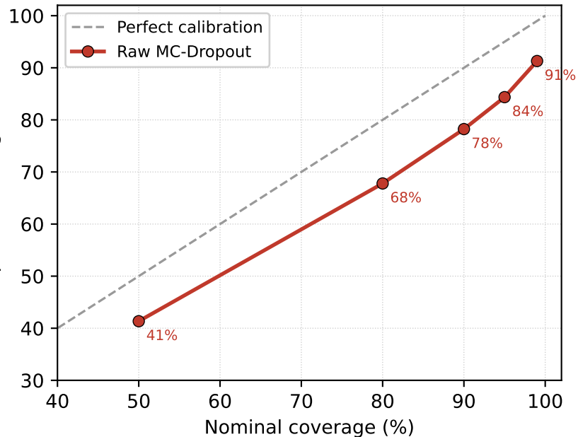
(a) Raw MC-Dropout reliability (17 test cells)
