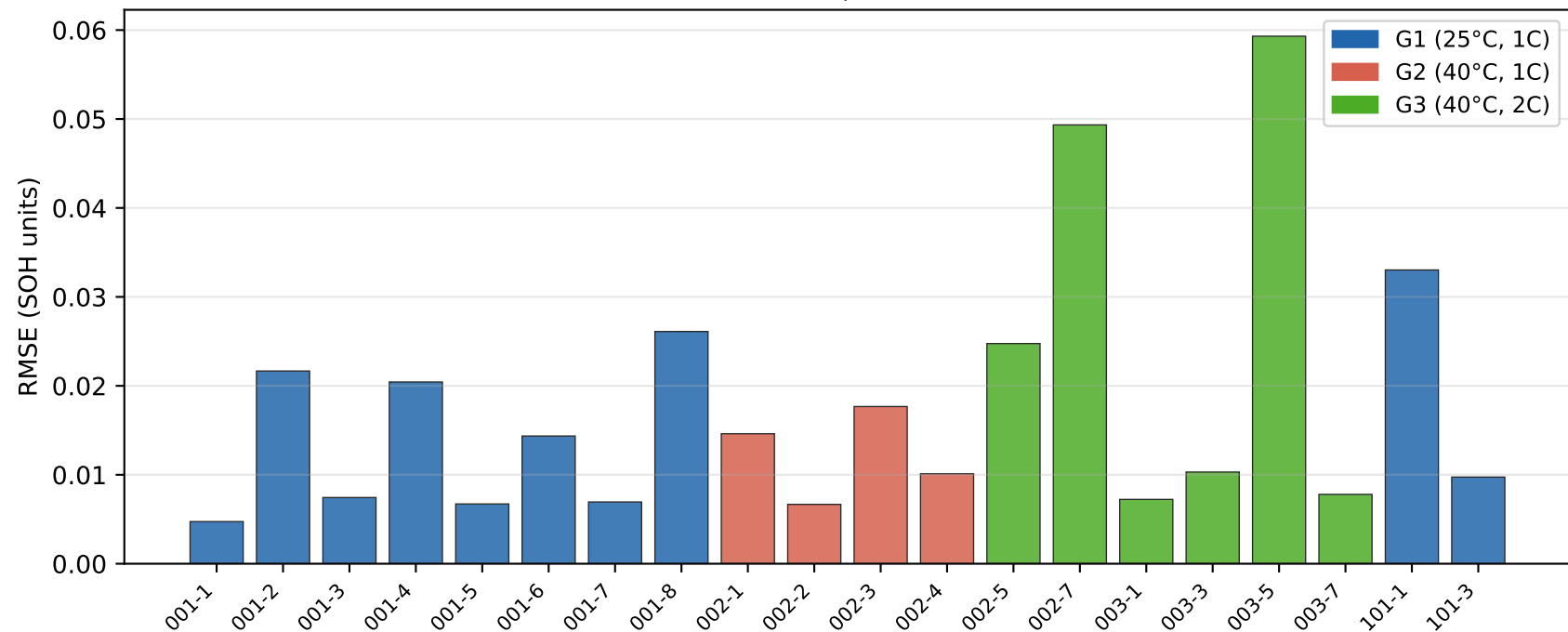
DE-LSTM baseline per cell (50% train)
