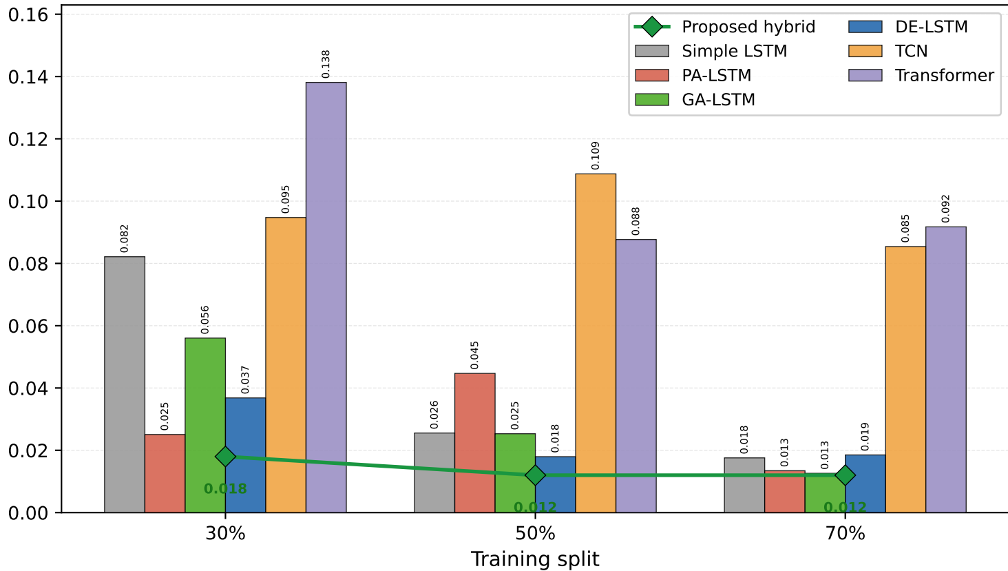
All-cell mean RMSE (SOH units)
